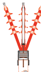
Series Heat Shrinkable Terminations Suitable for 3 Core Paper Insulated Lead Covered MIND Cable For 36 kV
