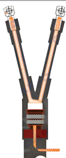
Series Heat Shrinkable Terminations Suitable for PVC/XLPE Cables upto 3.3kV.
