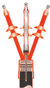
Series Heat Shrinkable Terminations Suitable for 3 Core XLPE/EPR Insulated Cables For 12kV
